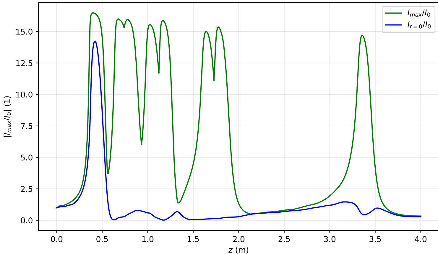
I_{max}(x = 0, y = 0, z)/I_0 , P_{in}=6.7P_{cr} , noisy input, artificial time
